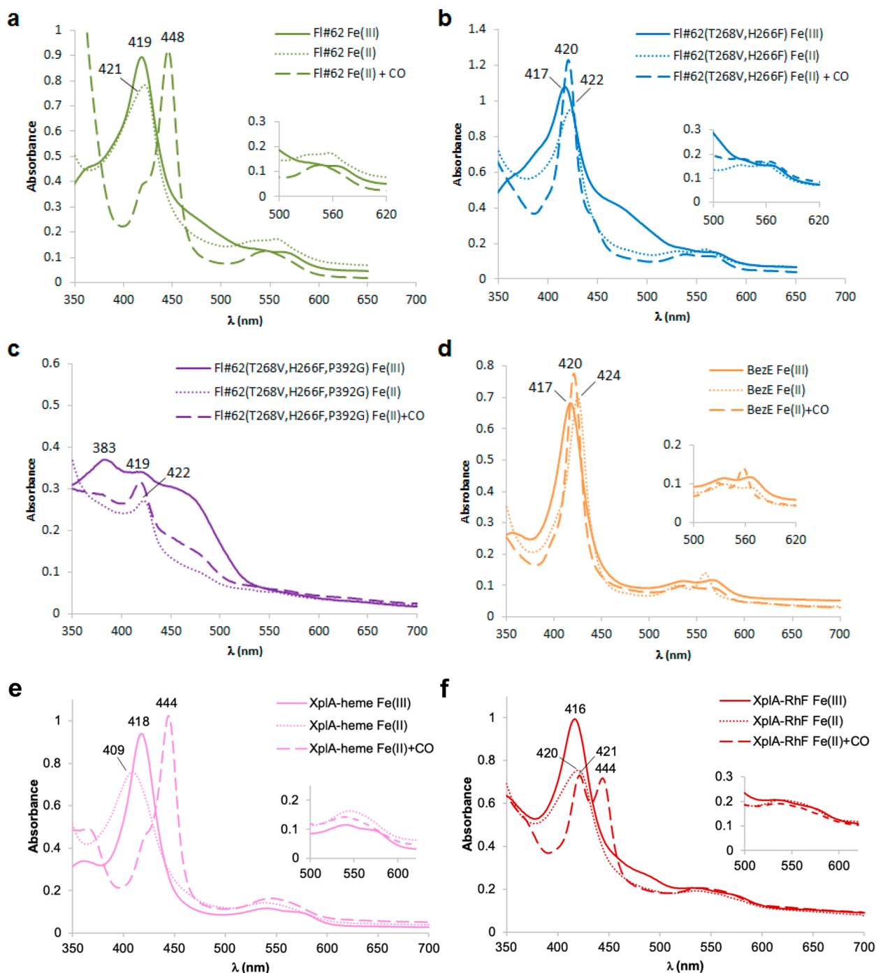
Figure 3. Electronic absorption spectra for (a) FL#62, (b) FL#62(H266F,T268V), (c) FL#62(H266F,T268V,P392G), (d) BezE, (e) XplA-heme, and (f) XplA-RhF in their ferric (solid line), ferrous (dotted line), and CO-bound form (dashed line). The inset shows the Q-band region.
