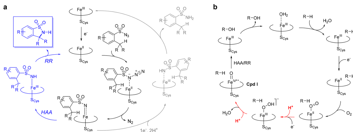
Figure 1. C–H amination vs C–H hydroxylation mechanism. (a) Proposed mechanism for cytochrome P450-catalyzed C–H amination of sulfonyl azides (blue) and the unproductive pathway leading to sulfonamide formation (gray). HAA = H atom abstraction; RR = radical rebound. (b) Catalytic cycle for P450-catalyzed monooxygenation (hydroxylation). The two proton transfer steps implicated in the formation of Compound I (Cpd I) are highlighted in red.
