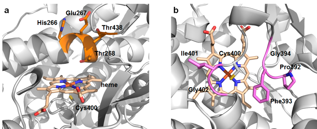
Figure 2. Distal and proximal regions surrounding the heme cofactor (stick model, wheat) in the crystal structure of cytochrome P450 BM3 heme domain (PDB 1BU7). (a) View of the P450 BM3 heme pocket highlighting Thr268 and other putative proton relay residues targeted by mutagenesis (orange). (b) View of proximal region of the enzyme highlighting the cysteine-ligand loop residues and other nearby residues targeted for mutagenesis (purple). The heme-ligating cysteine residue is also shown as stick model (gray).
